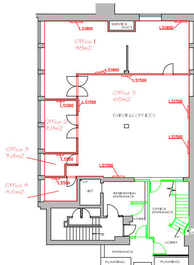
Sample CAD drawing showing radiator sizes and locations
